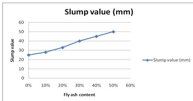
Chart- 3: Slump height of concrete mix
