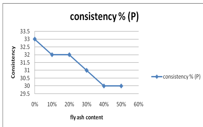
Chart- 1: Standard consistency of cement and fly ash mix
